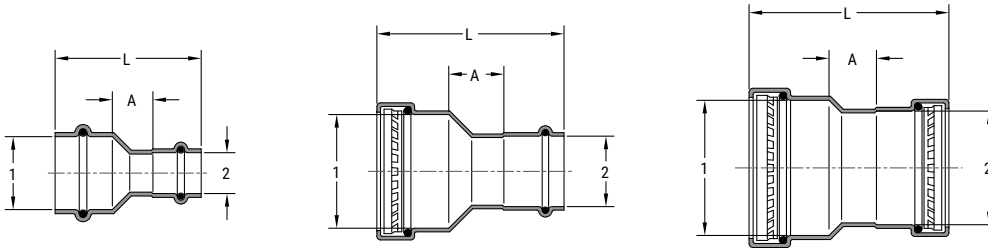
SP604R CU P X P RED COUPLING
