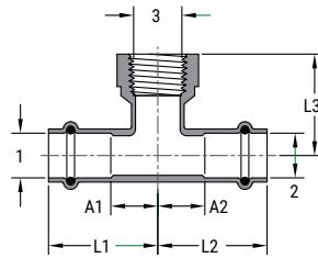
SP628 CU X P X P X FT ADPT TEE
