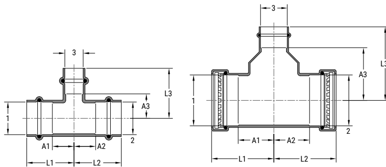
SP620R P x P x P Reducing Tee
